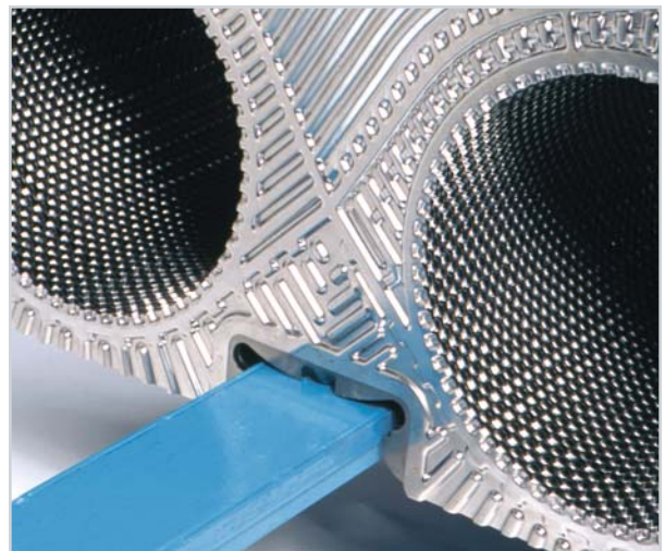
Closeup of Accu-Therm plates mounted on a unit's lower guide rail.
